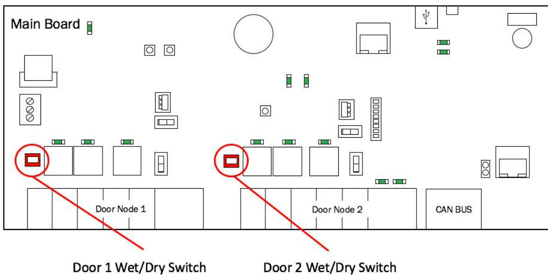
Figure 18 - ACS6000 Wet/Dry Door Contact Switches for Doors 1 and 2
