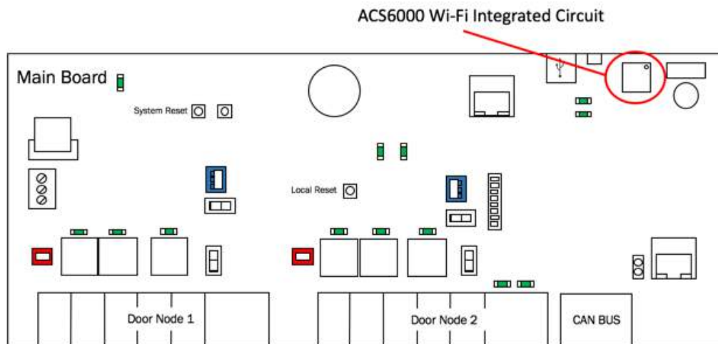
Figure 24 - ACS6000 Wi-Fi Integrated Circuit Location
